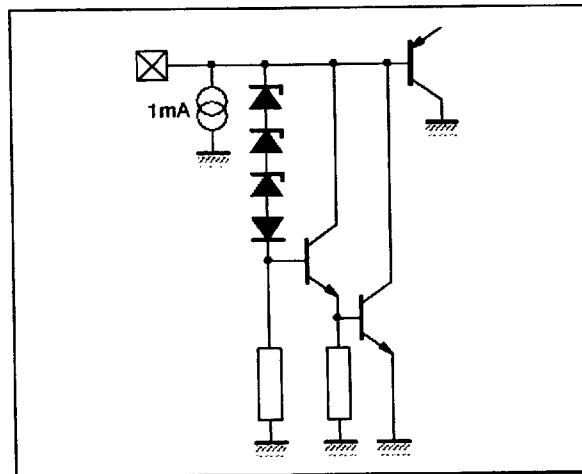
Pins : CCAS, H1, H2
