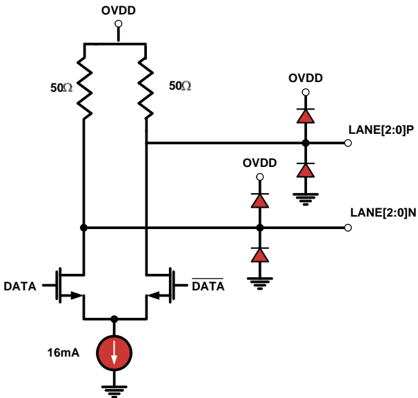
FIGURE 64. CML OUTPUTS
