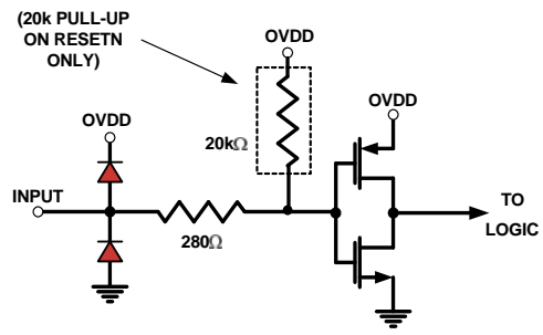
FIGURE 63. DIGITAL INPUTS
