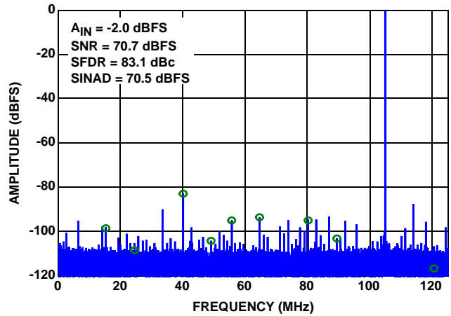
FIGURE 18. SINGLE-TONE SPECTRUM @ 105MHz (250MSPS)
