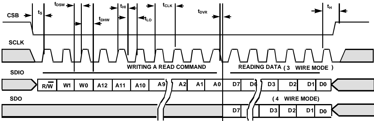
FIGURE 57. SPI READ
