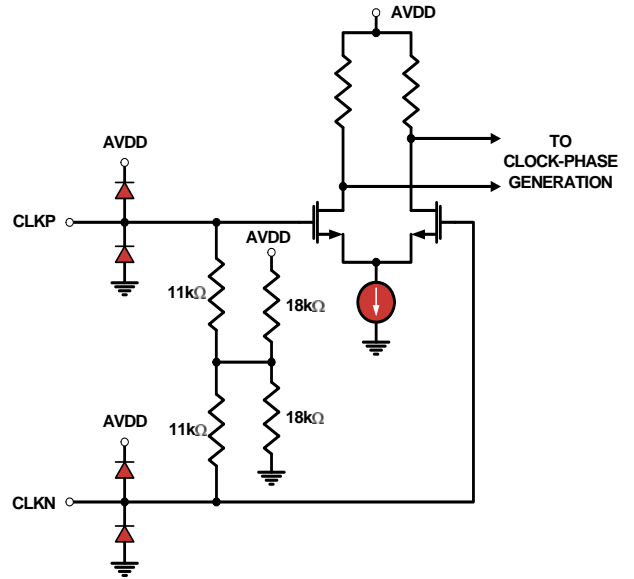
FIGURE 61. CLOCK INPUTS
