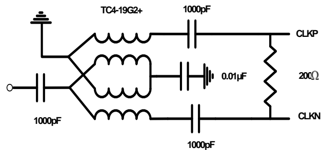
FIGURE 48. RECOMMENDED CLOCK DRIVE
