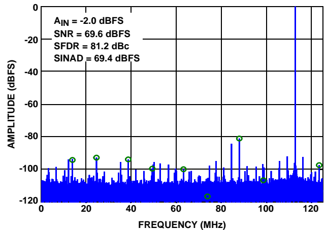
FIGURE 20. SINGLE-TONE SPECTRUM @ 363MHz (250MSPS)
