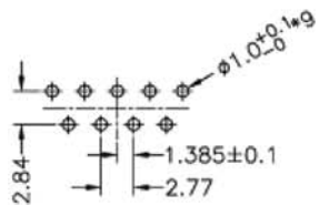
9 Pin Female Connector
