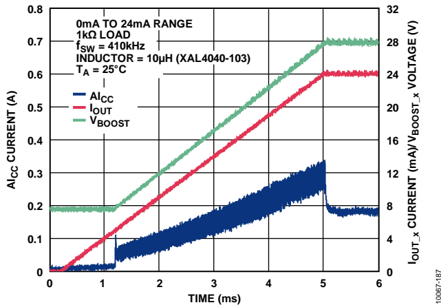
Figure 60. A_{I_{CC}} Current vs. Time for 24 mA Step Through 1 k \Omega Load with Slew Rate Control
