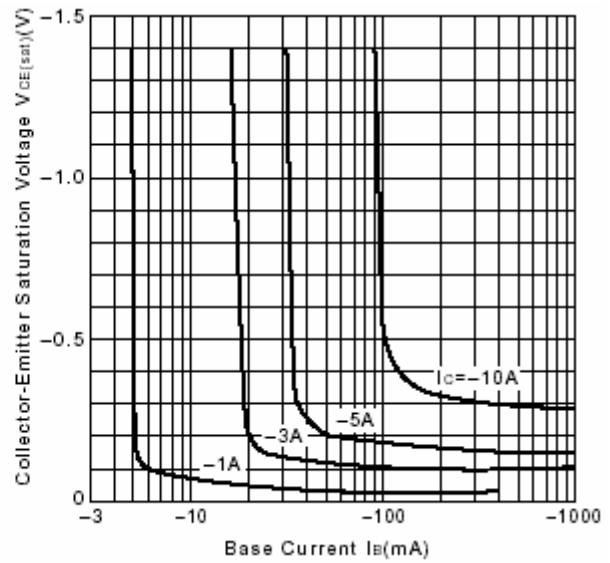
Fig.4 V_{CE(sat)}-I_B Characteristics
