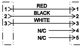
S3F5M WIRING DIAGRAM
