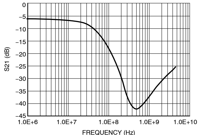
Figure 2. Typical Insertion Loss Characteristic
