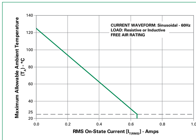
Figure 6: Maximum Allowable Ambient Temperature vs. On-State Current
