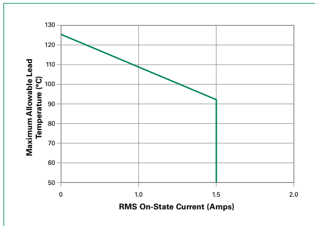
Figure 2: Maximum Allowable Lead/Tab Temperature vs. On-State Current
