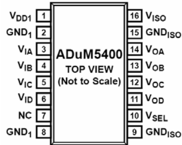
Figure 4. ADuM5400 Pin Configuration
