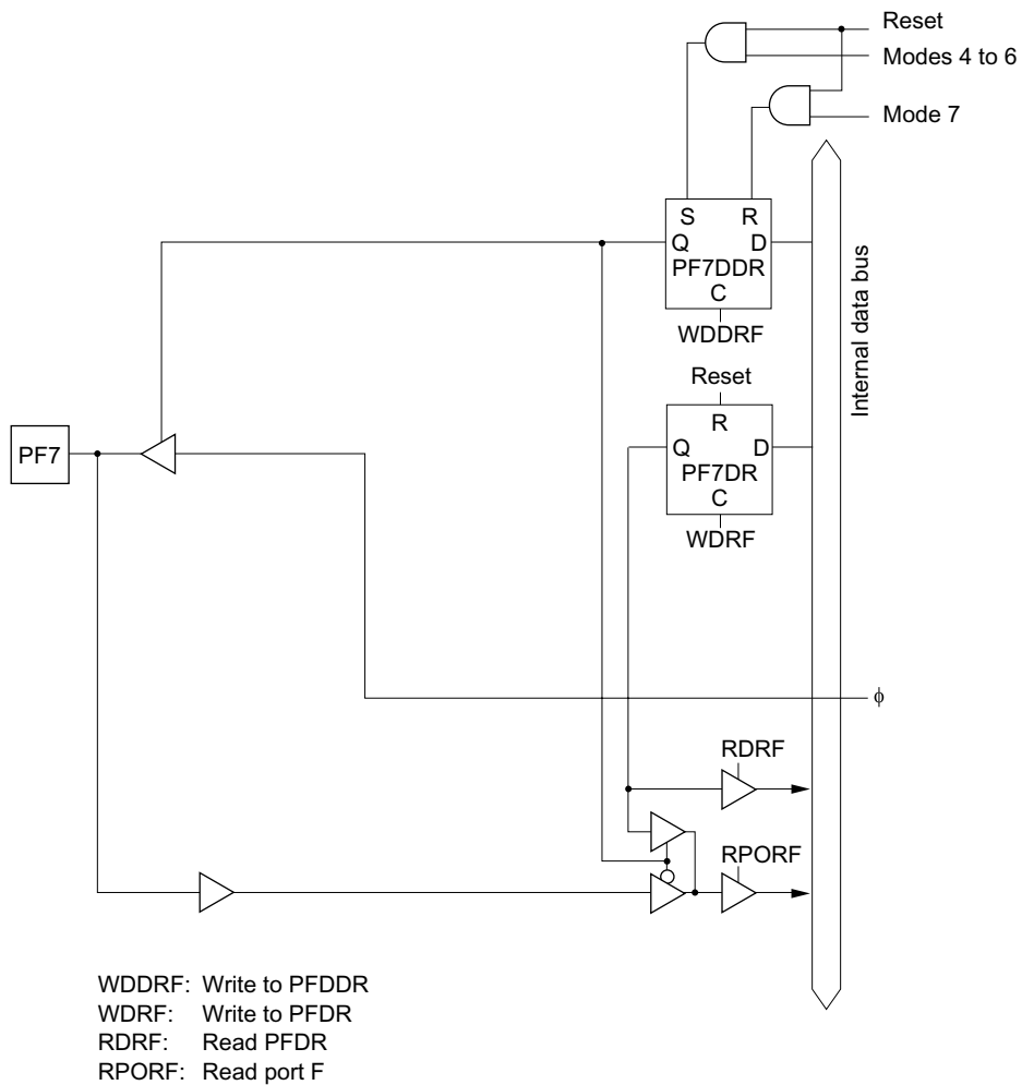
Figure C-10(h) Port F Block Diagram (Pin PF7)
