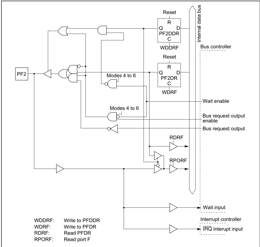
Figure C-10(c) Port F Block Diagram (Pin PF2)
