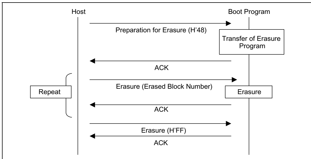
Figure 17-87 Erasure Sequence
