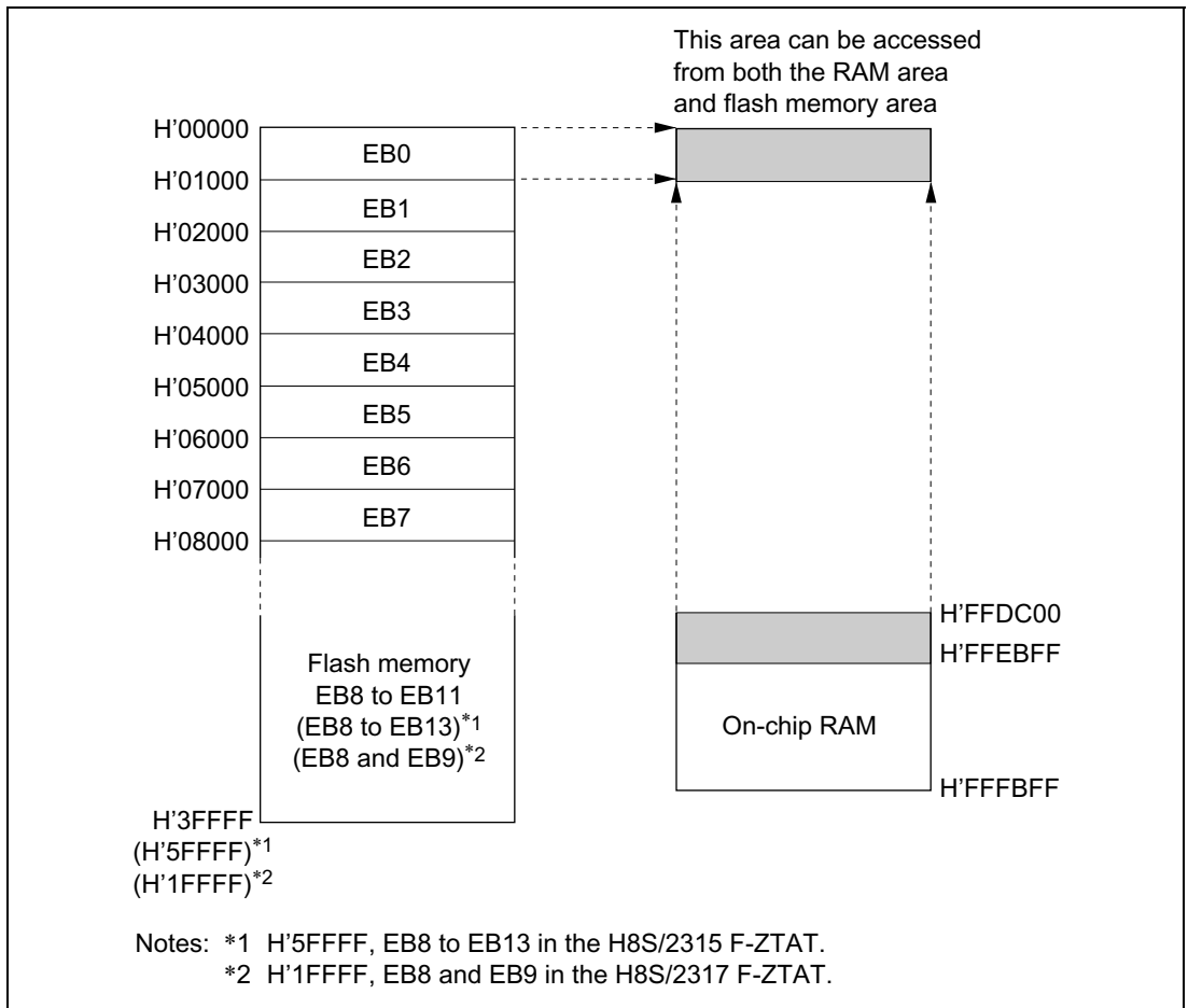
Figure 17-19 Example of RAM Overlap Operation
