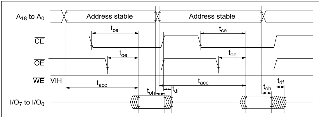
Figure 17-25 Timing Waveforms for \overline{CE}/\overline{OE} Clocked Read
