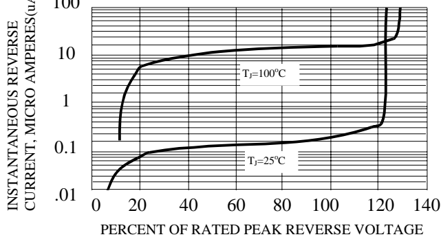
FIG. 4-TYPICAL REVERSE CHARACTERISTICS
