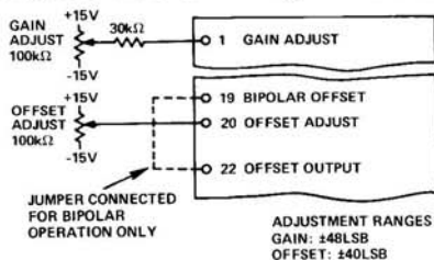
Figure 5. Adjustment Connections
