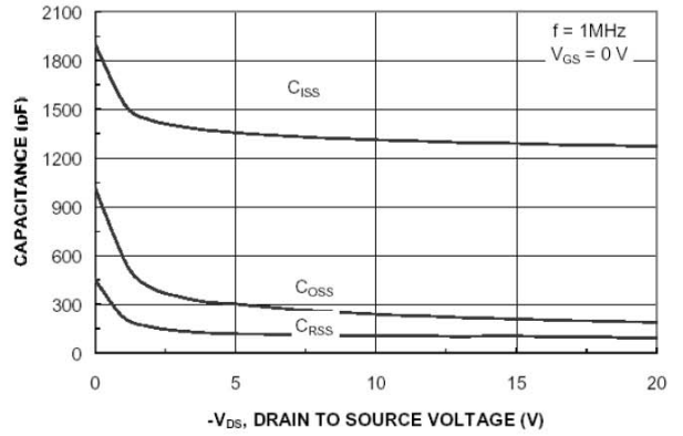
Figure 8. Capacitance Characteristic
