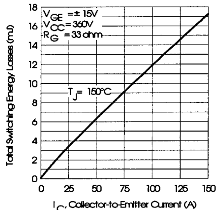
Fig. 10 - Typical Switching Losses vs. Collector-to-Emmitter Current
