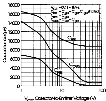
Fig. 8 - Typical Capacitance vs. Collector-to-Emmitter Voltage
