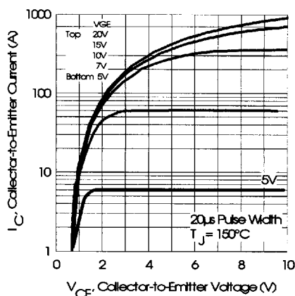
Fig. 2 - Typical Output Characteristics, T_J = 150^\circ\text{C}
