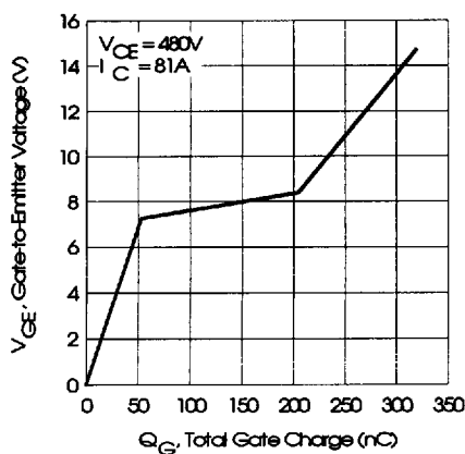
Fig. 7 - Typical Gate Charge vs. Gate-to-Emmitter Voltage
