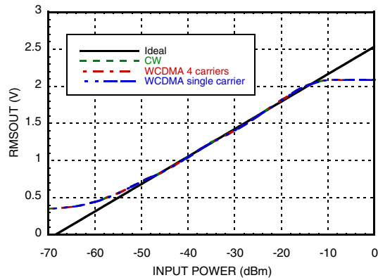
RMSOUT vs. Pin with Different Modulations @ 1900 MHz [1]
