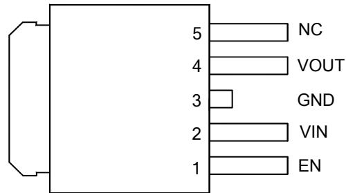
Figure 2. Pin Configuration of AZ39151 (Top View)
