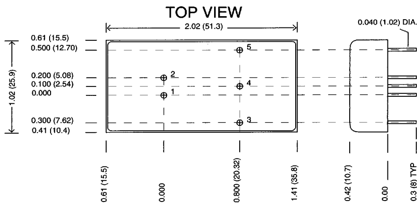
VPD SERIES CASE DRAWING NOMINAL CASE DIMENSIONS IN INCHES (MM) TOLERANCE X.XX ±0.020 (0.51), X.XXX —0.005 (0.13)
