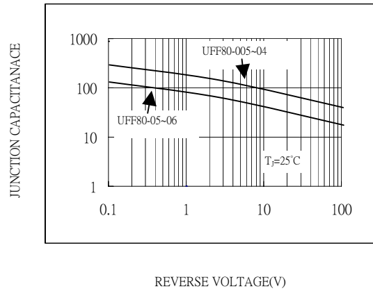
Fig.2-TYPICAL JUNCTION CAPACITANCE
