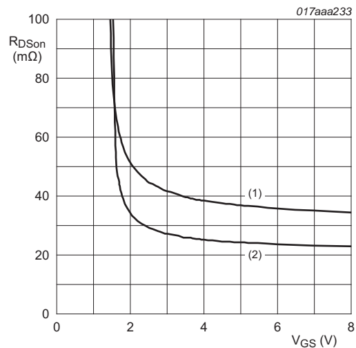
Fig 9. Drain-source on-state resistance as a function of gate-source voltage; typical values (1) T_j = 150 \text{ °C} (2) T_j = 25 \text{ °C}
