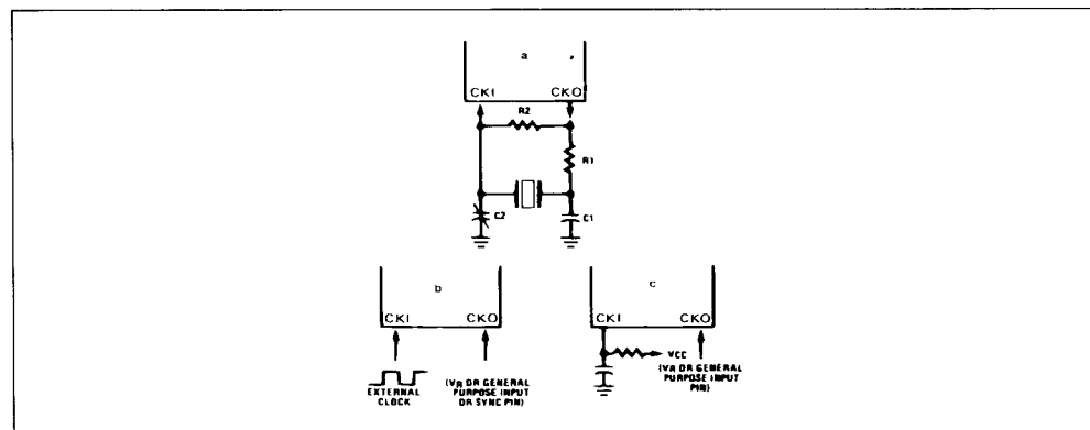
Figure 4 : ETL9420/L9421/L9422 Oscillator.
