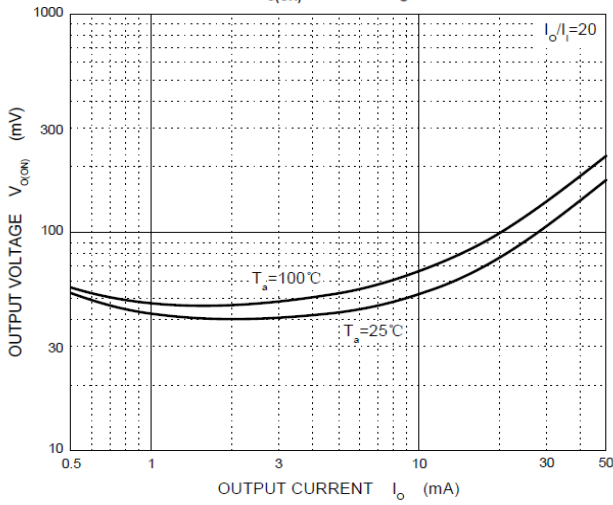
V_{(ON)} — I_o
