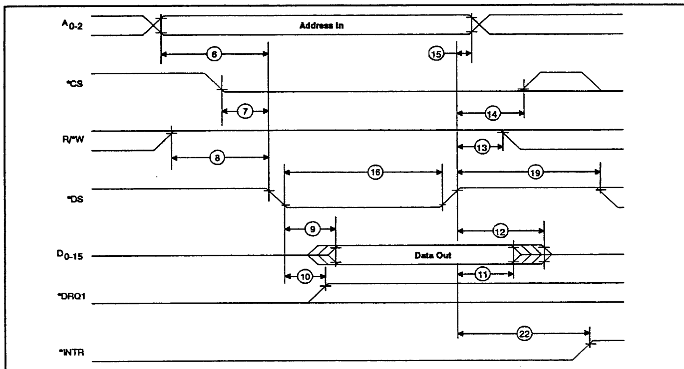
CPU Flow-Through Read Timing
