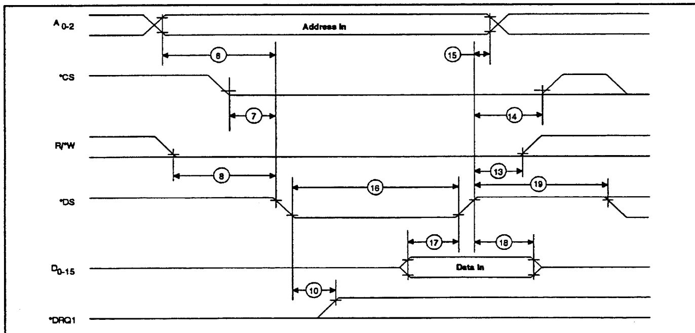
CPU Flow-Through Write Timing
