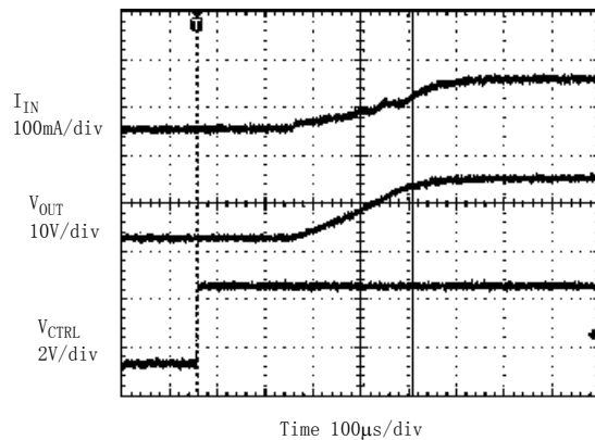
Figure 19. Soft Start Waveform VIN=3.6V, 4LEDS, ILED=20mA
