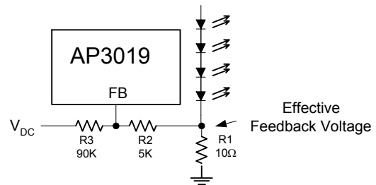
Figure 23. Dimming Control Using DC Voltage
