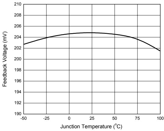
Figure 12. Feedback Voltage vs. Junction Temperature
