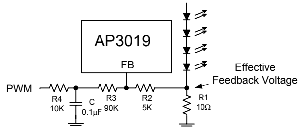
Figure 24. Dimming Control Using a Filtered PWM Voltage
