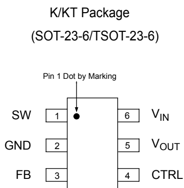
Figure 2. Pin Configuration of AP3019 (Top View)
