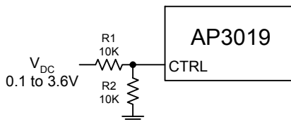
Figure 21. Dimming Control Using a DC Voltage in CTRL Pin
