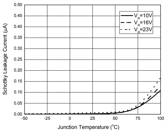
Figure 14. Schottky Leakage Current vs. Junction Temperature
