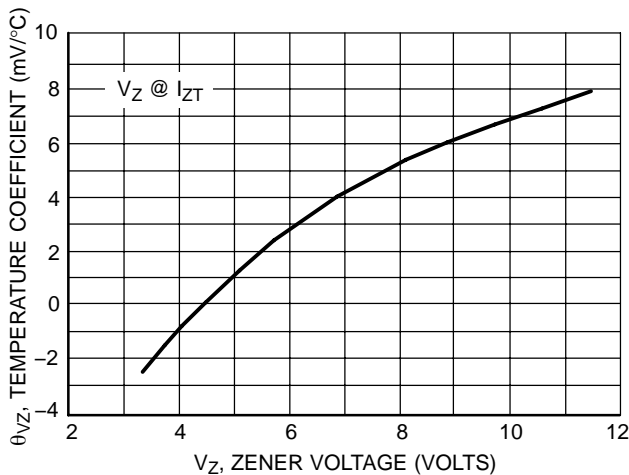
Figure 4. Zener Voltage - To 12 Volts
