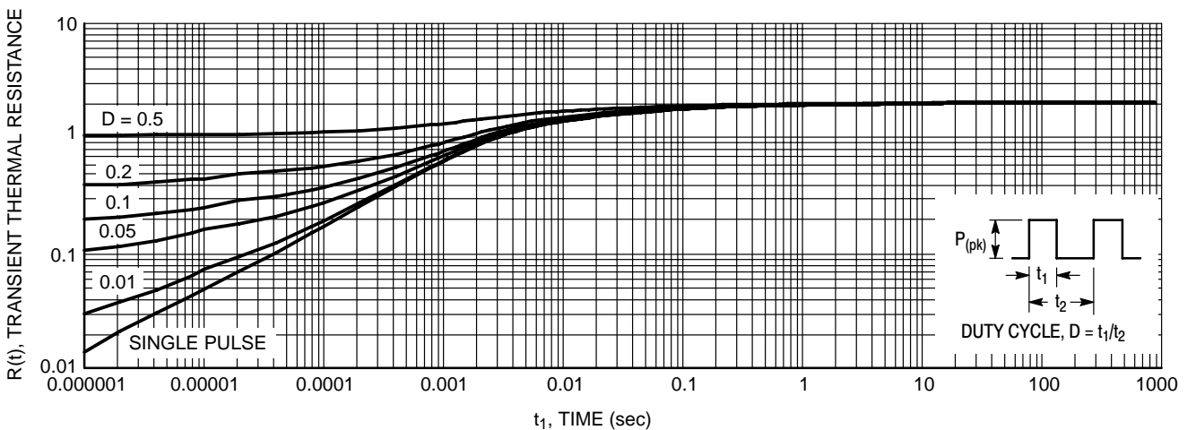
Figure 10. Thermal Response Junction-to-Case
