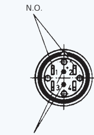
LED-terminals
