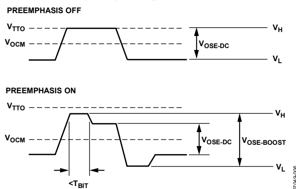
Figure 28. Preemphasis Pulse Response
