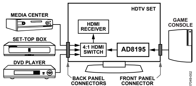
Figure 2. Typical AD8195 Application for HDTV Sets
