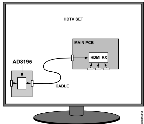
Figure 29. AD8195 as a Front Panel Buffer for an HDTV
