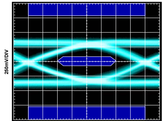
Figure 13. Tx Eye Diagram at TP3, PE = 6 dB (Cable = 10 Meters, 24 AWG)
