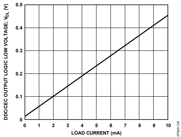
Figure 25. DDC/CEC Output Logic Low Voltage ( V_{OL} ) vs. Load Current
