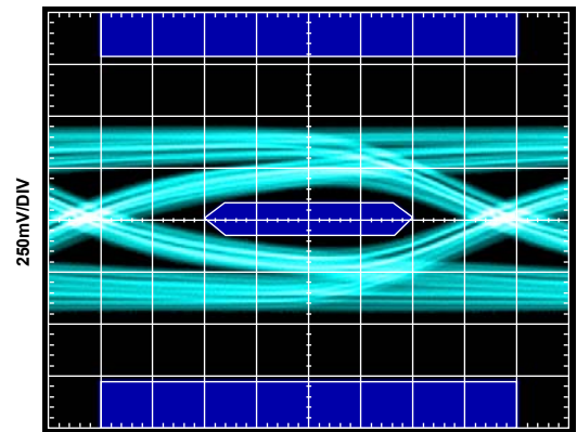
Figure 12. Tx Eye Diagram at TP3, PE = 0 dB (Cable = 6 Meters, 24 AWG)
