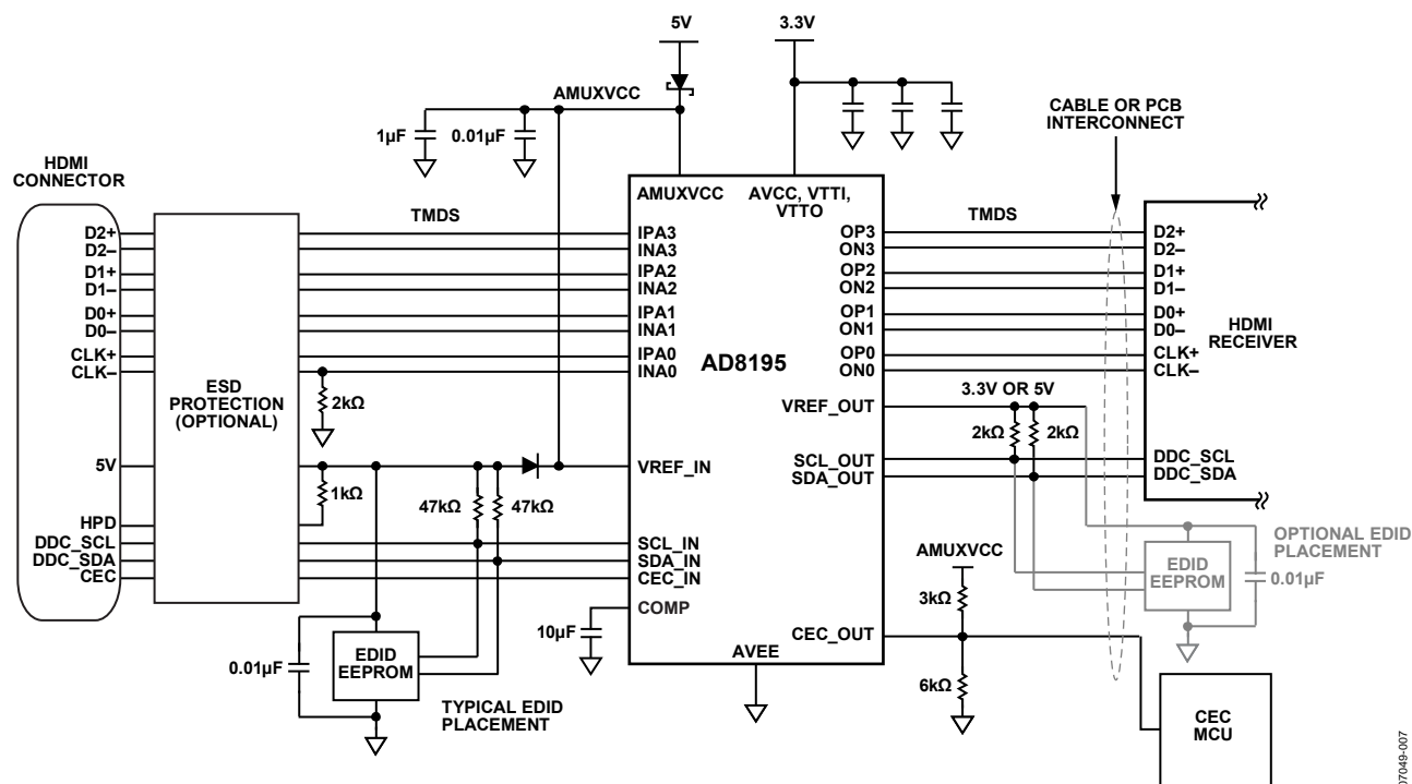
Figure 30. AD8195 Typical Application Simplified Schematic
