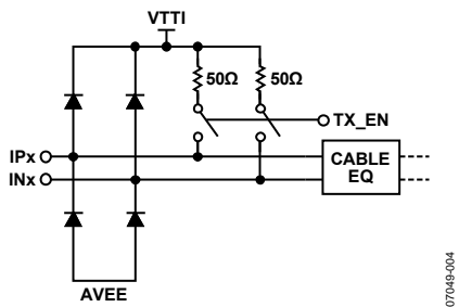
Figure 26. High Speed Input Simplified Schematic
