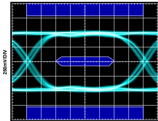
Figure 10. Tx Eye Diagram at TP2, PE = 0 dB
