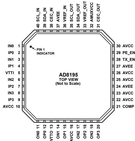
Figure 3. Pin Configuration
