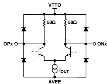
Figure 27. High Speed Output Simplified Schematic
