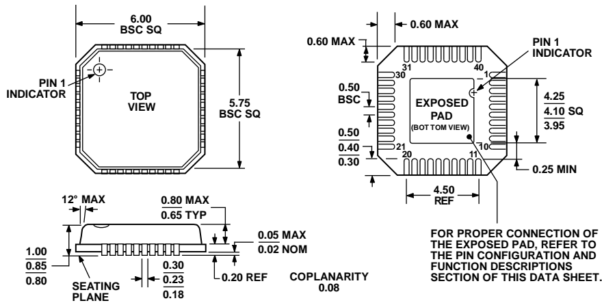
Figure 32. 40-Lead Lead Frame Chip Scale Package [LFCSP_VQ] 6 mm × 6 mm Body, Very Thin Quad (CP-40-1) Dimensions shown in millimeters
