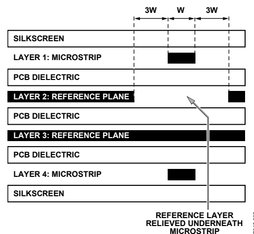
Figure 31. Example Board Stack-Up
