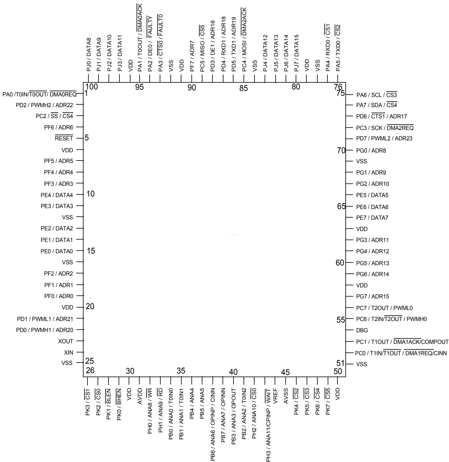
Figure 5. ZNEO Z16F Series in 100-Pin Low-profile Quad Flat Package (LQFP)
