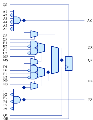
FIGURE 4. Logic Cell
