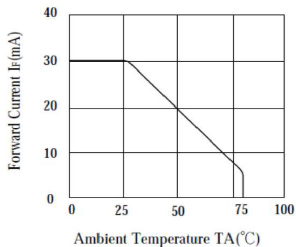
MAX FORWARD CURRENT Vs. AMBIENT TEMPERATURE
