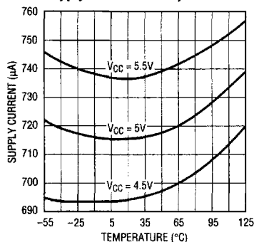
LTC1454 Supply Current vs Temperature
