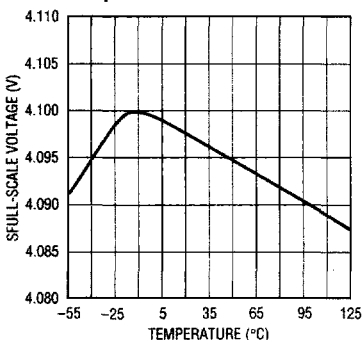
LTC1454 Full-Scale Voltage vs Temperature
