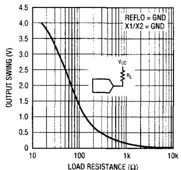
LTC1454 Output Swing vs Load Resistance
