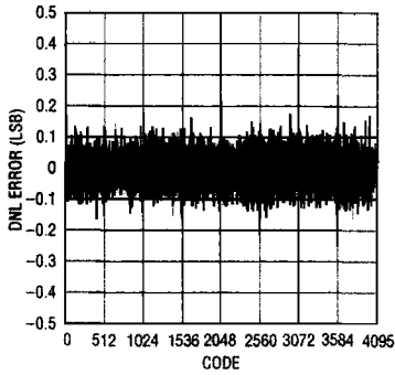
LTC1454 Differential Nonlinearity
