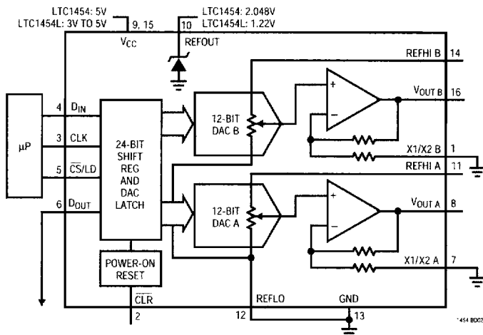
Functional Block Diagram: Dual 12-Bit Rail-to-Rail DAC
