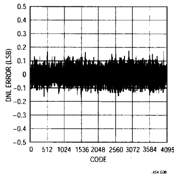
Differential Nonlinearity vs Input Code
