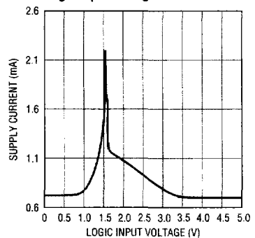
LTC1454 Supply Current vs Logic Input Voltage
