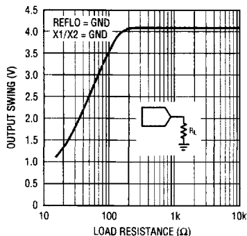
LTC1454 Output Swing vs Load Resistance
