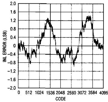
LTC1454 Integral Nonlinearity
