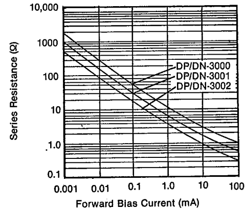
R_S vs. I_F Characteristics
