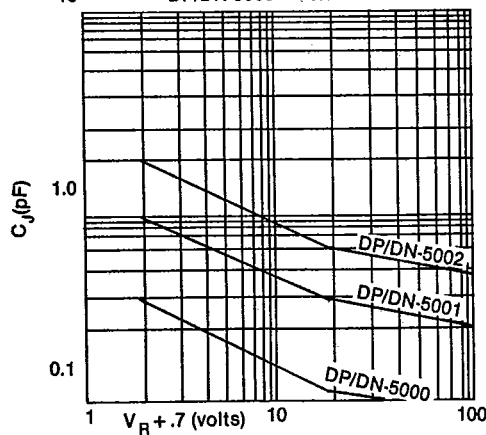
Capacitance/Voltage Characteristics DP/DN-5000 Series
