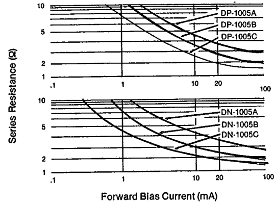
R_S vs. I_F Characteristics
