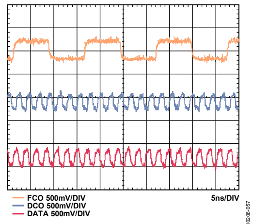
Figure 58. LVDS Output Timing Example in Reduced Range Mode
