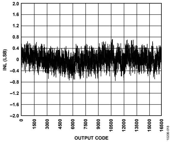
Figure 19. INL, f_{IN} = 9.7 MHz, f_{SAMPLE} = 65 MSPS
