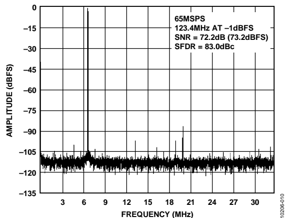
Figure 11. Single-Tone 16k FFT with f_{IN} = 123.4 MHz, f_{SAMPLE} = 65 MSPS
