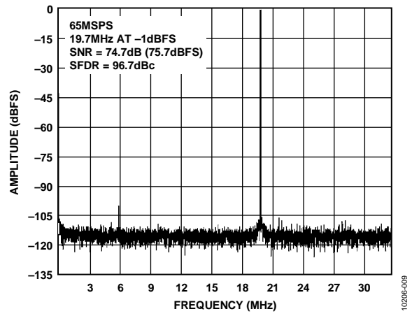
Figure 9. Single-Tone 16k FFT with f_{IN} = 19.7 MHz, f_{SAMPLE} = 65 MSPS
