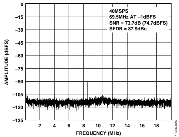
Figure 25. Single-Tone 16k FFT with f_{IN} = 69.5 MHz, f_{SAMPLE} = 40 MSPS
