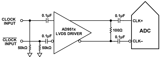
Figure 53. Differential LVDS Sample Clock (Up to 520 MHz)
