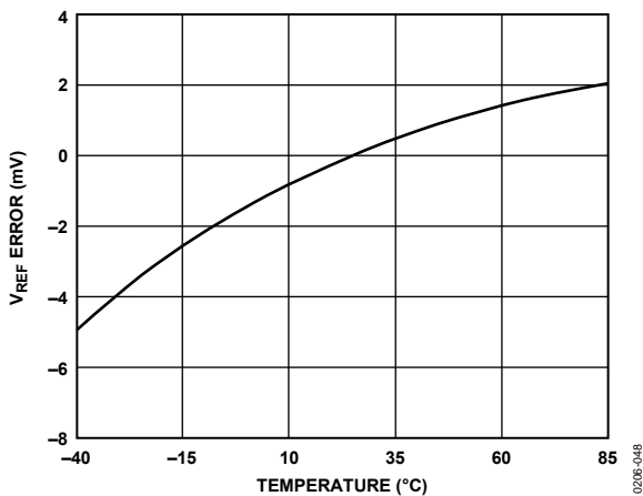
Figure 49. Typical VREF Drift
