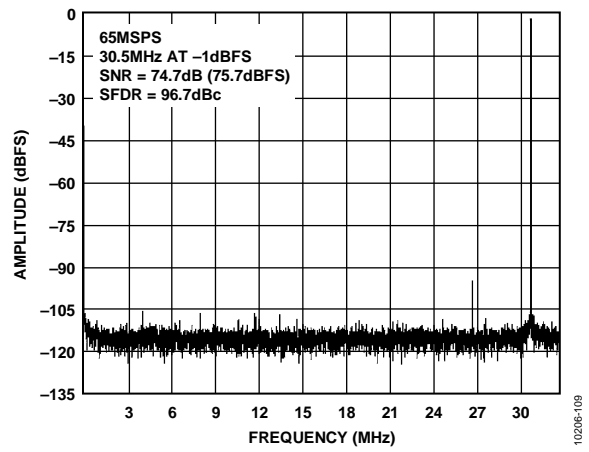
Figure 10. Single-Tone 16k FFT with f_{IN} = 30.5 MHz, f_{SAMPLE} = 65 MSPS
