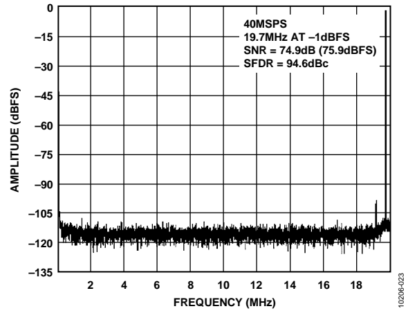
Figure 24. Single-Tone 16k FFT with f_{IN} = 19.7 MHz, f_{SAMPLE} = 40 MSPS
