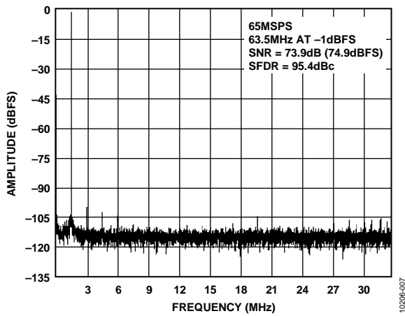
Figure 7. Single-Tone 16k FFT with f_{IN} = 63.5 MHz, f_{SAMPLE} = 65 MSPS
