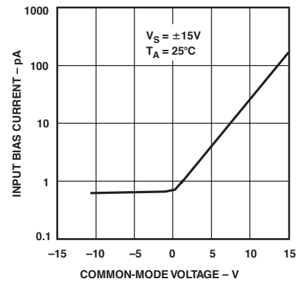
TCP 9. OP282 Input Bias Current vs. Common-Mode Voltage
