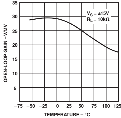
TPC 2. Open-Loop Gain (V/mV) vs. Temperature
