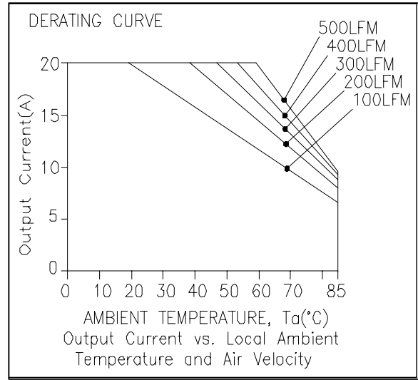
Derating curve under worst case input
