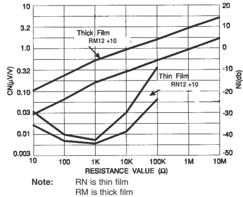
Current Noise
