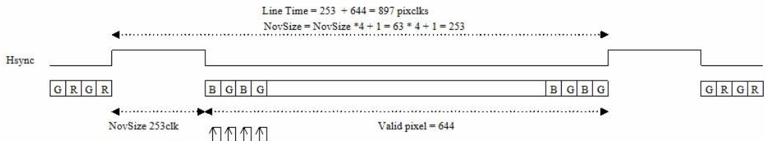
Figure 3.7 Inter-line timing of W.O.I
