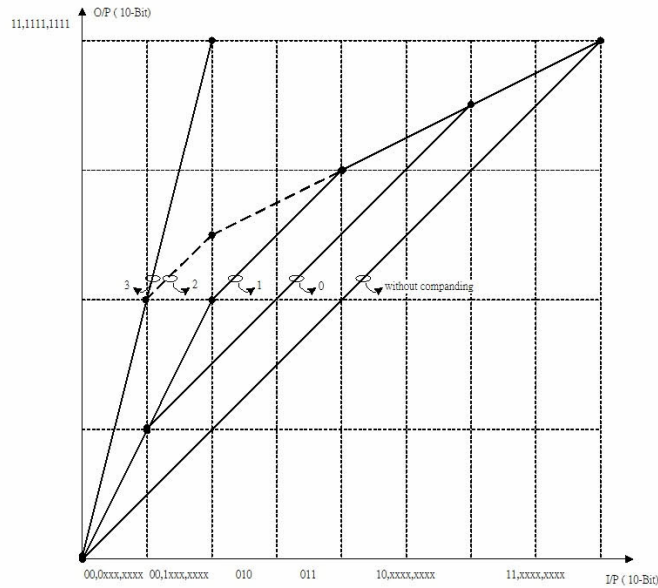
Figure 3.2 Companding curves program by Comband_EnH and Comband_Sel
