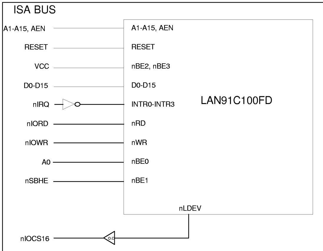
FIGURE 14 - LAN91C100FD ON ISA BUS
