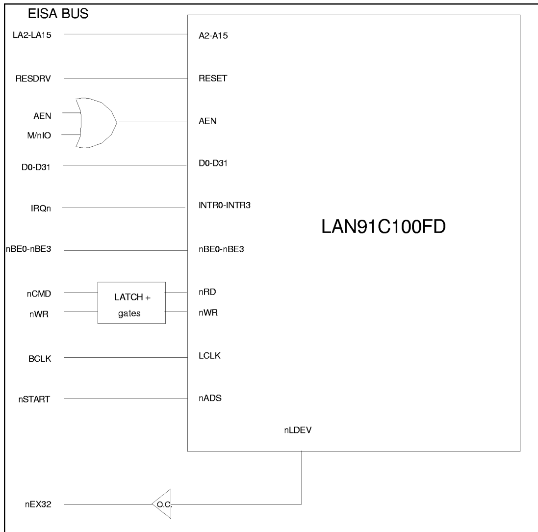
FIGURE 15 - LAN91C100FD ON EISA BUS
