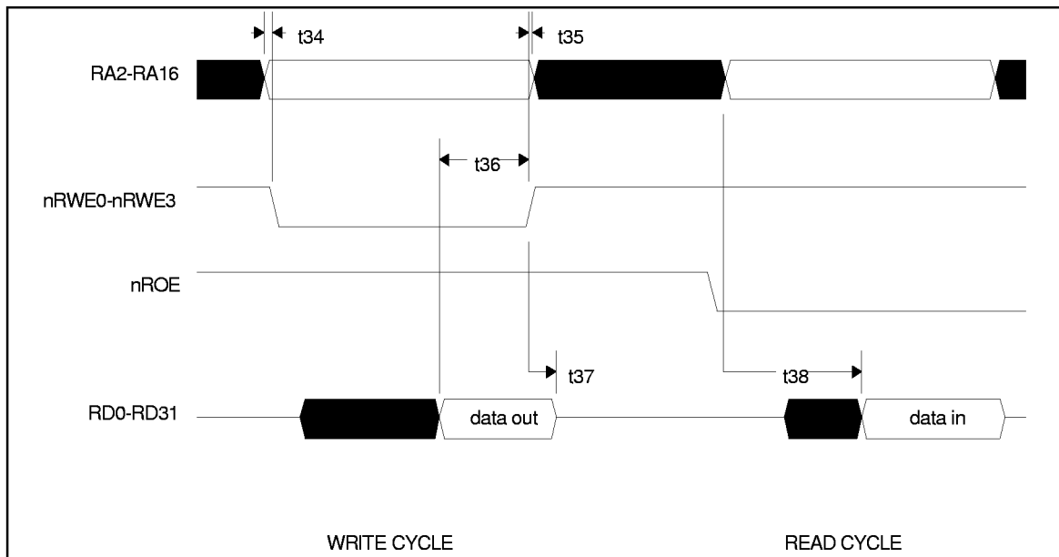
FIGURE 24 - SRAM INTERFACE
