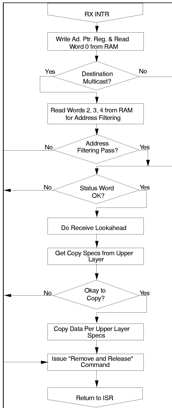
FIGURE 7 - RX INTR
