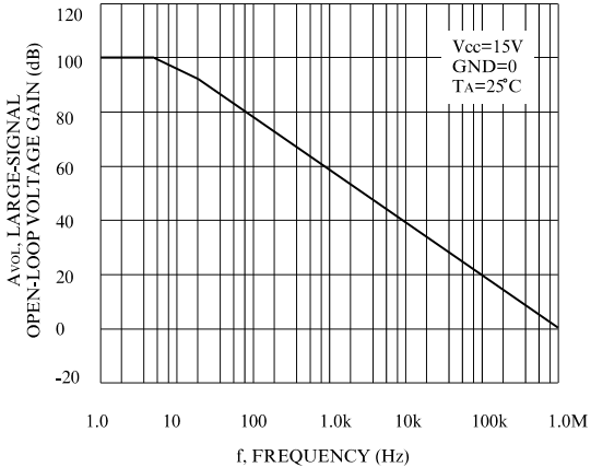
Figure 2. Open-Loop Frequency
