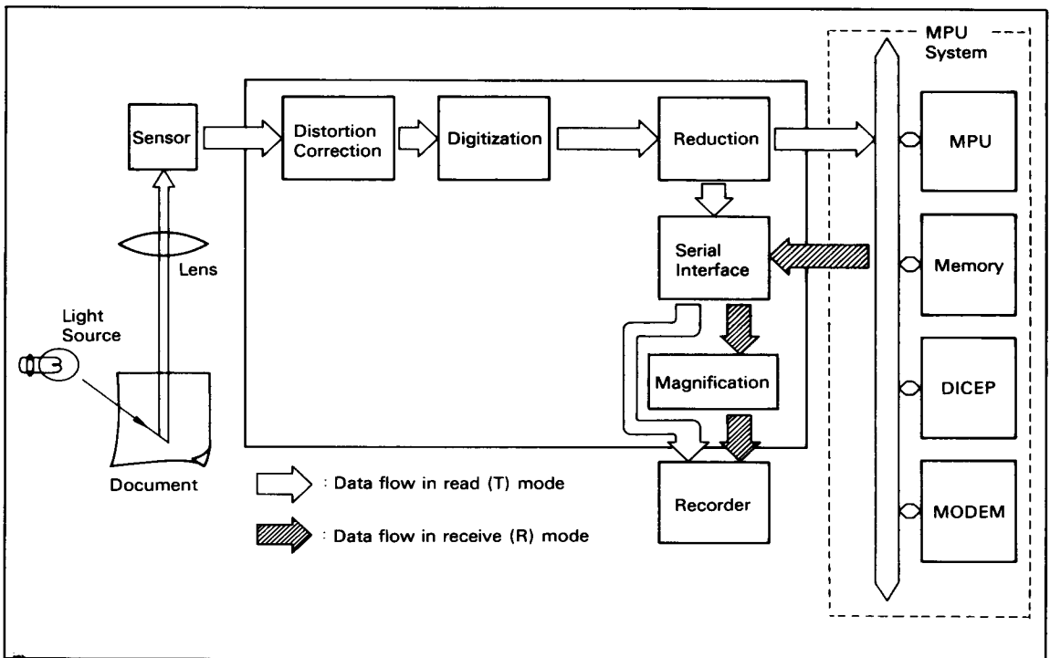
Figure 1 DIPP Function
