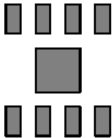
Minimum Footprint , \theta_{JA} = 75^{\circ}\text{C}/\text{W}
