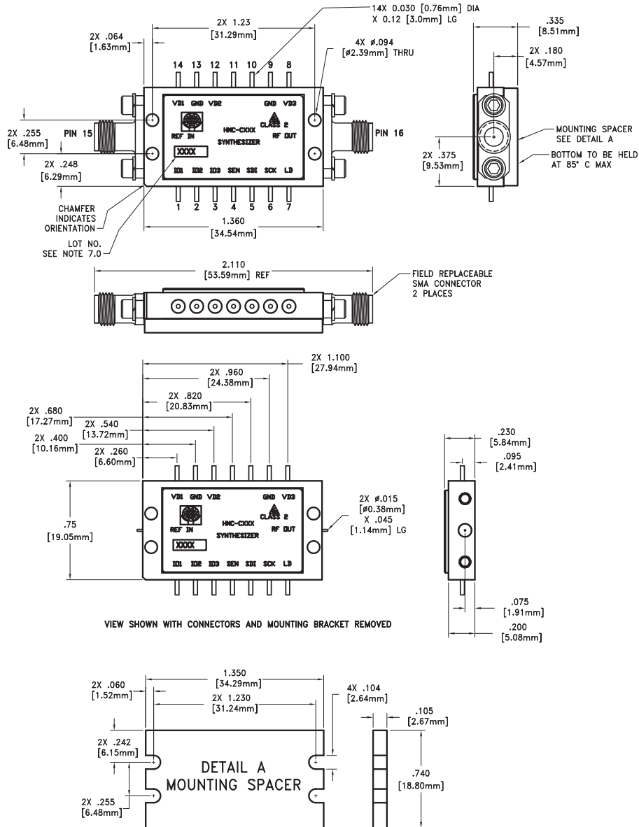
C-20 Package Outline Drawing
