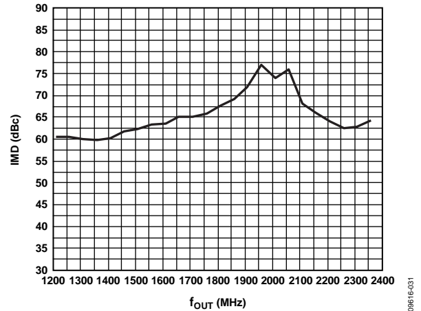
Figure 111. IMD in Mix-Mode vs. f_{OUT} at 2.4 GSPS
