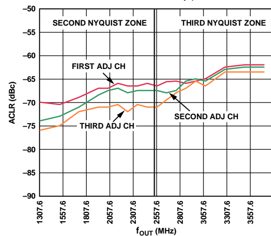
Figure 38. Single-Carrier WCDMA ACLR vs. f_{OUT} , f_{DAC} = 2457.6 MSPS
