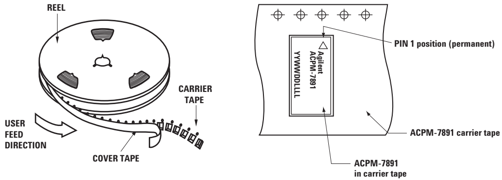
CARRIER TAPE
