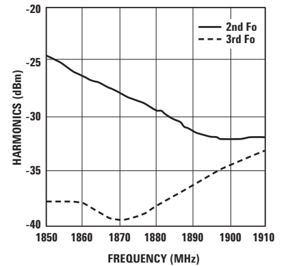
Figure 15. 2 nd and 3 rd Harmonic Performance (PCS Band, Pin = 0 dBm, Pout = 32 dBm, Vdd = 3.0V).
