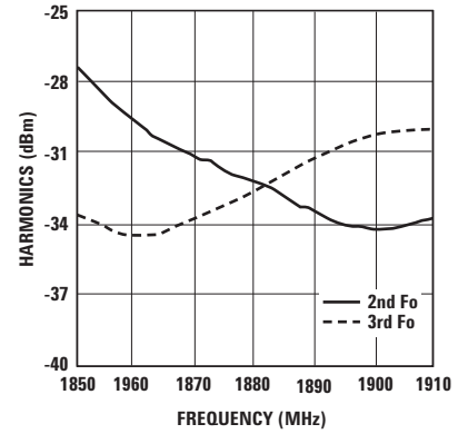
Figure 12. 2 nd and 3 rd Harmonic Performance (PCS Band, Pin = 0 dBm, Pout = 32 dBm, Vdd = 3.5V).
