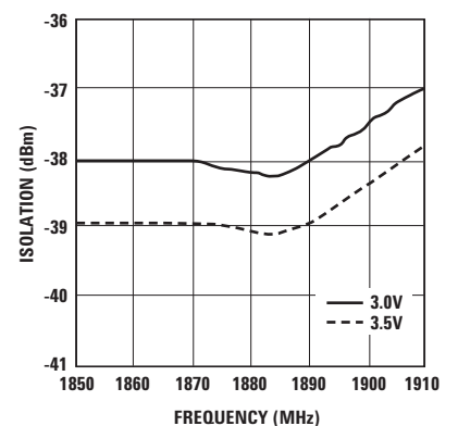
Figure 18. Isolation Performance (PCS Band, Pin=4 dBm, Vapc=0.2V).
