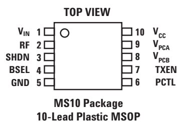
Figure C1. LTC-1758-2 Pinout.
