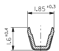
SECT. B-B (SCALE 10:1)
