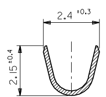
SECT. C-C (SCALE 10:1)
