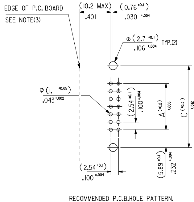
RECOMMENDED P.C.B.HOLE PATTERN.
