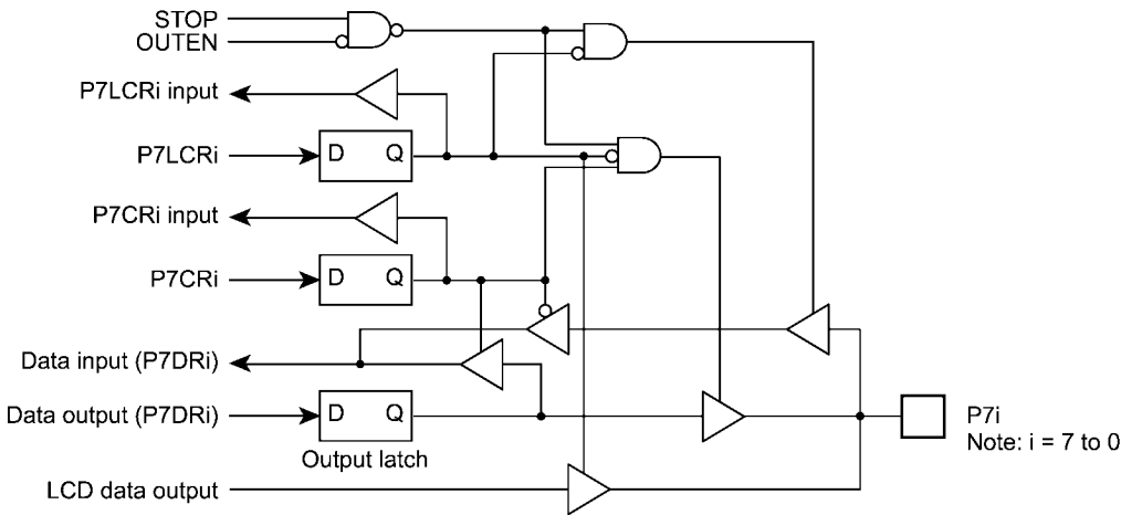
Figure 5-7 Port P7
