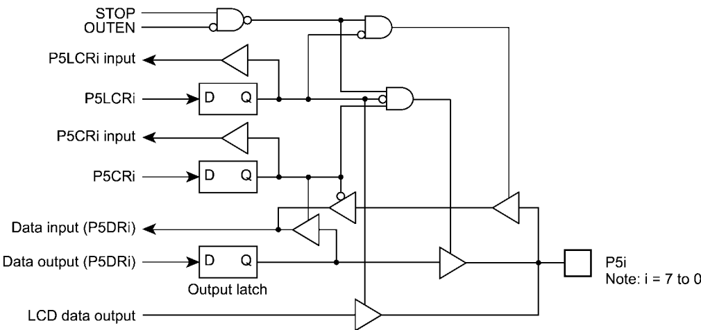
Figure 5-5 Port P5
