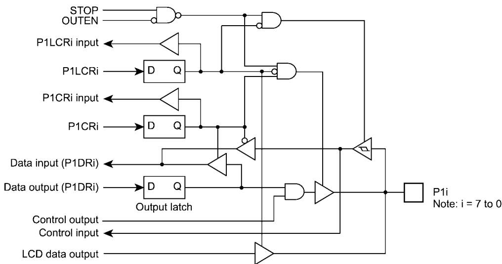
Figure 5-2 Port P1
