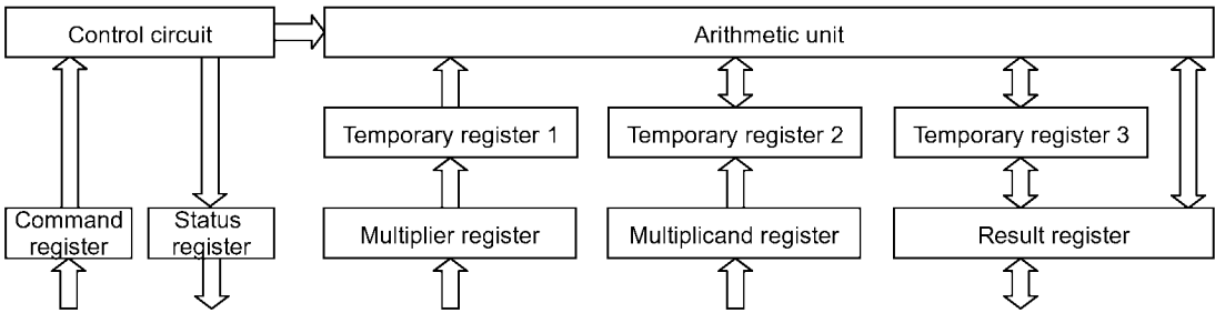
Figure 17-1 MAC Unit
