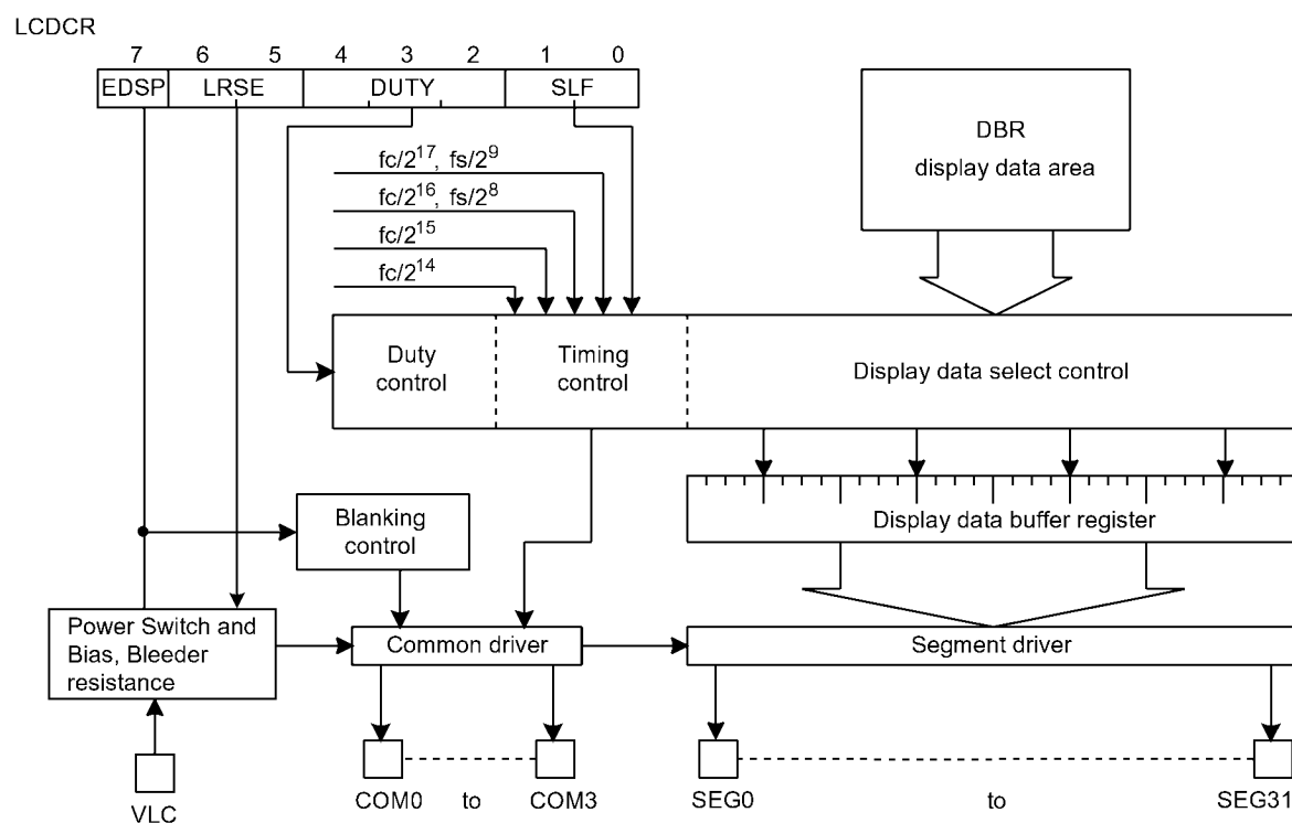
Figure 15-1 LCD Driver
