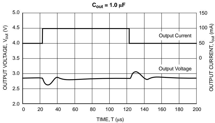
Figure 15. Load Transient Response ( V_{out} = 2.8 V , t_r = t_f = 5.0 \mu s , V_{in} = 3.8 V )
