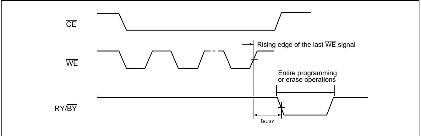
(9) RESET, RY/ \overline{\text{BY}} Timing Diagram
