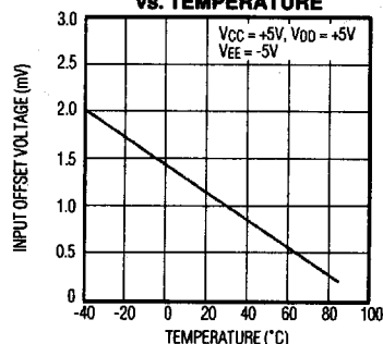
INPUT OFFSET VOLTAGE vs. TEMPERATURE
